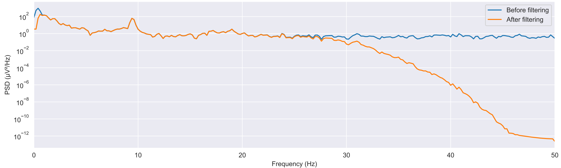
PSD Before vs After Filtering: Subject 6, Epoch 5, Fpz-Cz
